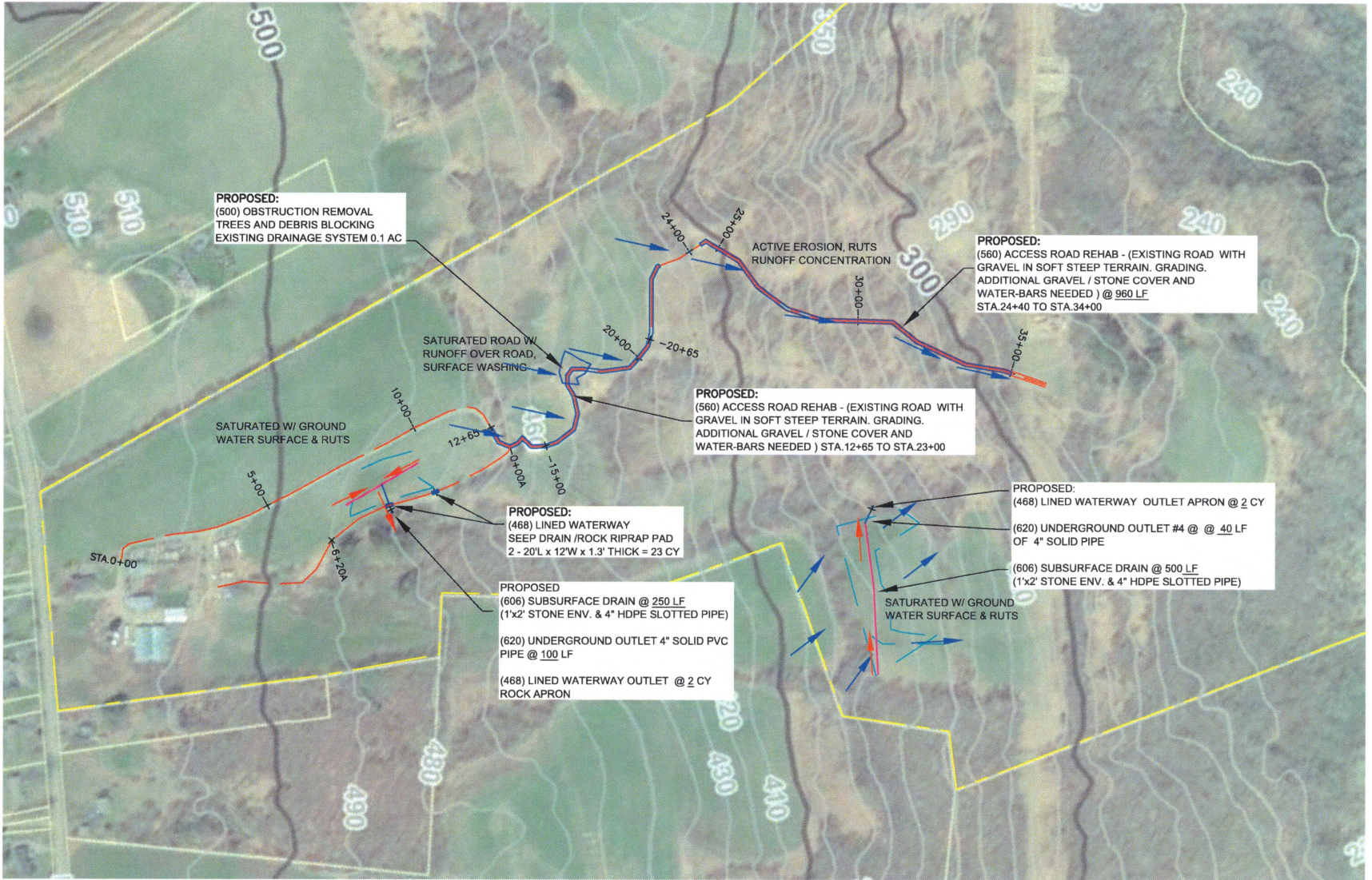
PROPOSED I&E FIELD DRAINAGE SITE PLAN VIEW
